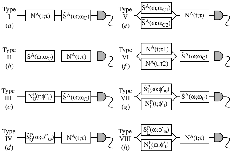
FIGURE 11.7 Linear filter description of type I to type VIII devices.
