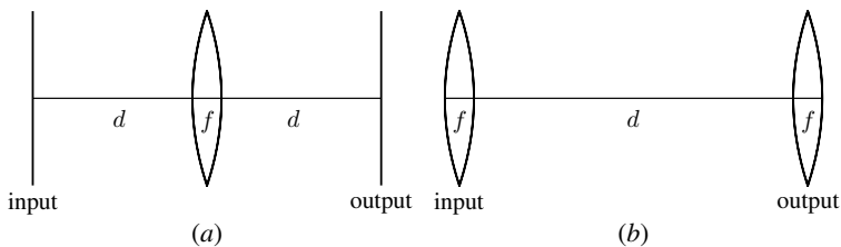
FIGURE 1.3 Two optical realizations of the fractional Fourier transformer.
