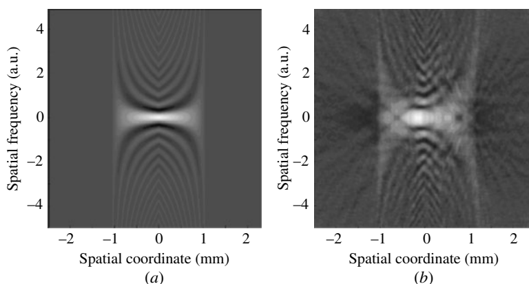
FIGURE 4.17 (a) Theoretical WDF of a single slit. (b) Experimental result for the tomographic reconstruction of the WDF of the same slit.
