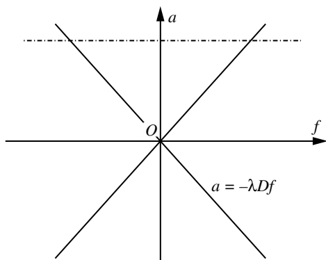
FIGURE 2.1 Schematic PSO representation. The AF along the line a = -\lambda Df corresponds to the intensity spectra \tilde{I}_D(f) at distance D from the reference plane. The integration of formula (2.37) is to be performed along lines parallel to the f axis.
