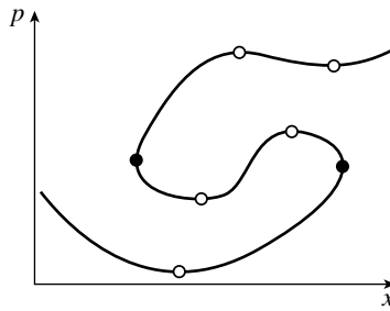
FIGURE 8.5 Vertical segments (indicated by black dots) of the PSC correspond to position caustics, while horizontal segments (indicated by open dots) correspond to momentum caustics.
