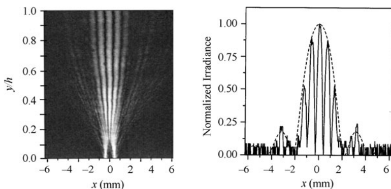
FIGURE 4.13 RDW showing the evolution of the field diffracted by a double slit. (a) Experimental result. (b) Cross section of the RWD showing the intensity profile near the Fraunhofer region. For comparison purposes, the theoretical sinc envelope of the Young fringes is also shown by the dotted line.
