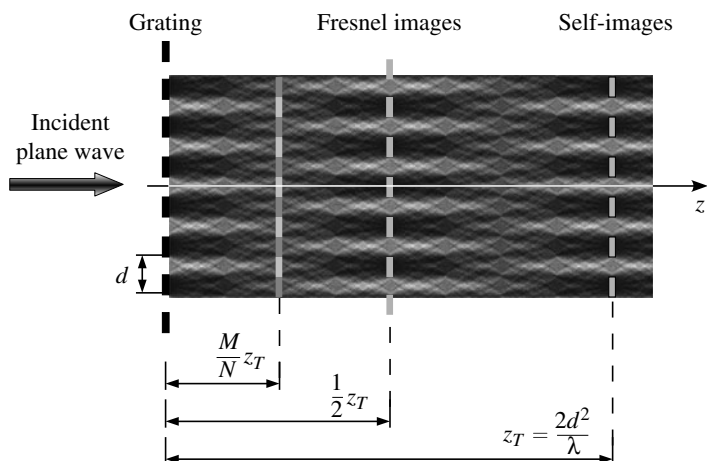
FIGURE 9.3 Configuration to observe the Talbot effect and the fractional Talbot effect.
