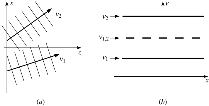
FIGURE 9.1 Interference in phase space: (a) Two propagating coherent plane waves and (b) the corresponding phase-space diagram.
