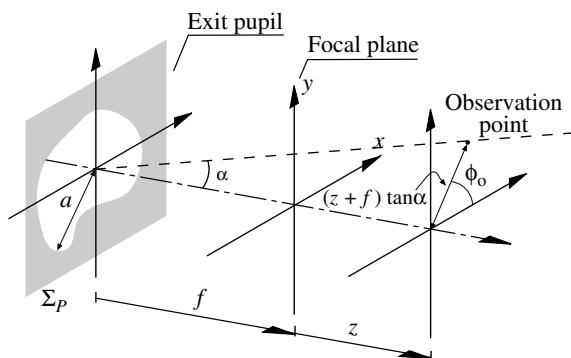
FIGURE 4.9 Trajectories in image space.
