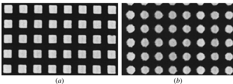
FIGURE 4.30 Gray-scale display of the irradiance distribution to be achromatized: (a) Monochromatic pattern for \lambda_o = 546.1 nm. (b) Broadband (Hg lamp) irradiance distribution.
