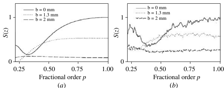
FIGURE 4.20 SR versus defocus for circular pupils with pupil function t(x) = \text{rect}(x/h) - \text{rect}(x/b) : (a) Computer simulation; (b) experimental results. Again, the projection angle \theta = p\pi/2 .
