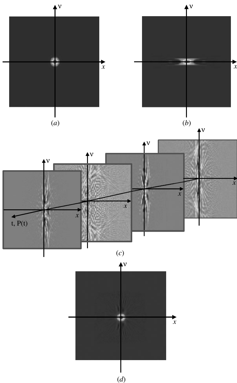
FIGURE 6.10 The Wigner transform of (a) Gaussian signal, (b) Gaussian signal after being low passed with a spectral rectangular aperture, (c) the low passed signal being multiplied by the time-varying random decoding mask, and (d) the resulting Wigner distribution of the time-averaged decoded signal.
