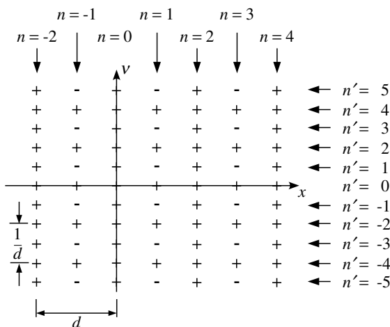
FIGURE 9.6 The PSD of the comb function. The \delta functions with a positive (+) sign are interlaced with \delta functions with a negative (−) sign.
