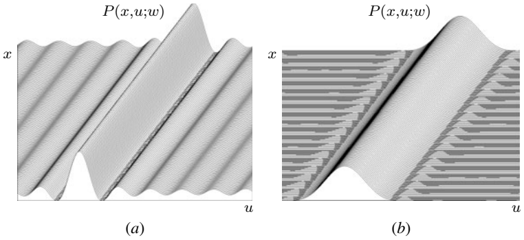
FIGURE 1.2 Numerical simulation of the (pseudo) Wigner distribution P(x, u; w) \simeq W(x, u) = \delta(u - hx) of the spherical wave f(x) = \exp(i\pi hx^2) , for the case that w(\frac{1}{2}x') is (a) a rectangular window and (b) a Hann(ing) window.
