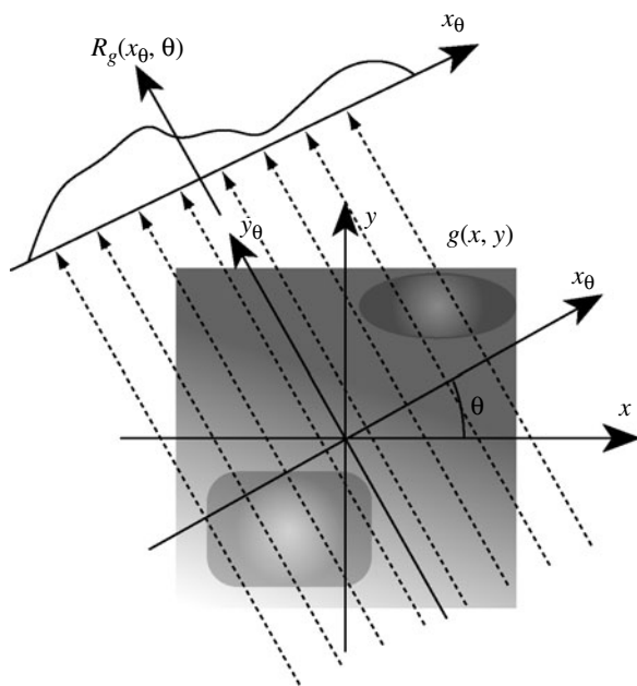
FIGURE 4.1 Projection scheme for the definition of the Radon transform.
