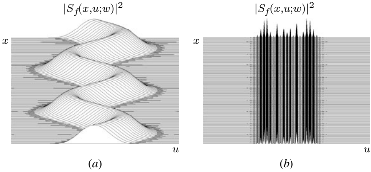
FIGURE 1.5 Spectrogram of a sinusoidal FM signal \exp[i[2\pi u_0 x + a_1 \sin(2\pi u_1 x)]] with (a) a medium-sized window, leading to a space-frequency representation with smearing, and (b) a long window, leading to a pure frequency representation.
