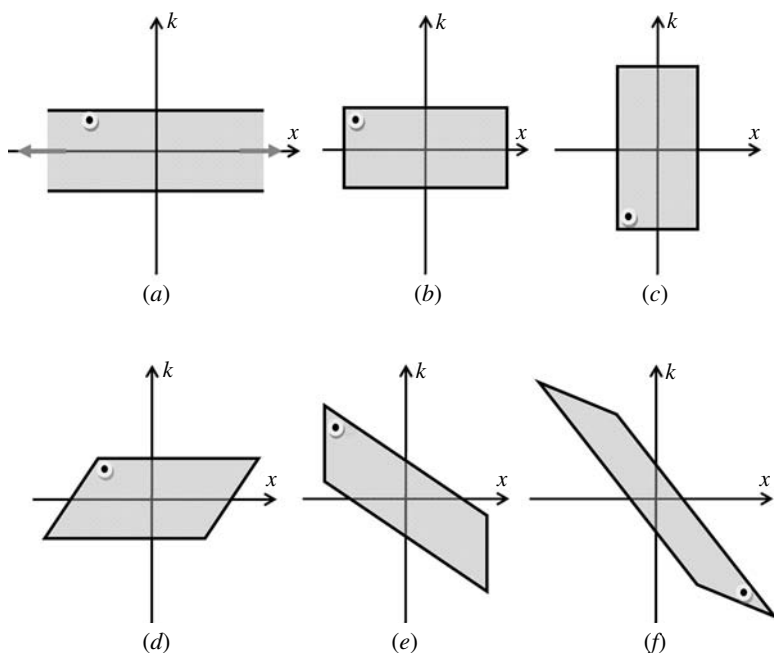
FIGURE 10.1 The PSD of a signal (a) having finite bandwidth and therefore an infinite spatial support, (b) having approximately finite spatial support and finite bandwidth, (c) which is a Fourier transform of signal represented in part b, (d) which is a Fresnel transform of the signal represented in part b, (e) which is a signal represented in part b after being multiplied by a chirp function, and (f) which is a linear canonical transform of the signal represented in part b.
