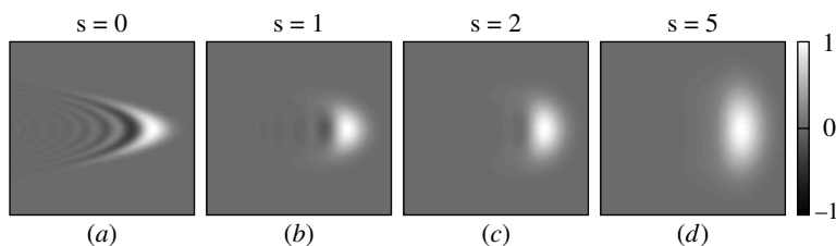
FIGURE 11.2 Smoothed Wigner functions P_s of a pulse with Gaussian spectrum and third-order spectral phase for (a) s = 0 , (b) s = 1 , (c) s = 2 , and (d) s = 5 . Part a corresponds to the Wigner function and part c corresponds to a spectrogram.
