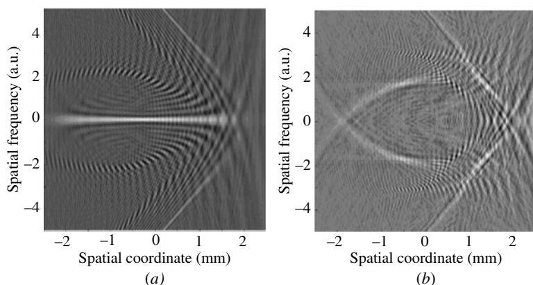
FIGURE 4.18 (a) Theoretical WDF of a binary grating with a linearly increasing spatial frequency. (b) Experimental tomographic reconstruction of the WDF of the same grating.
