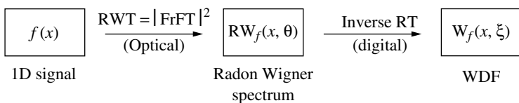
FIGURE 4.15 Diagram of the proposed hybrid optodigital method.
