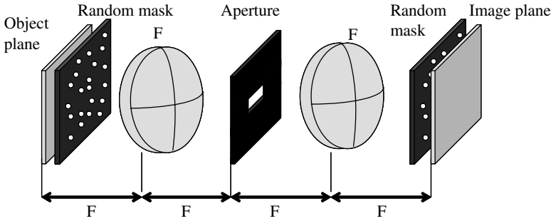
FIGURE 6.2 Schematic sketch of the imaging setup.
