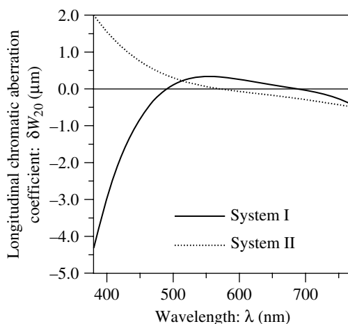
FIGURE 4.23 Longitudinal chromatic aberration coefficient associated with the two different correction states of the system under study.
