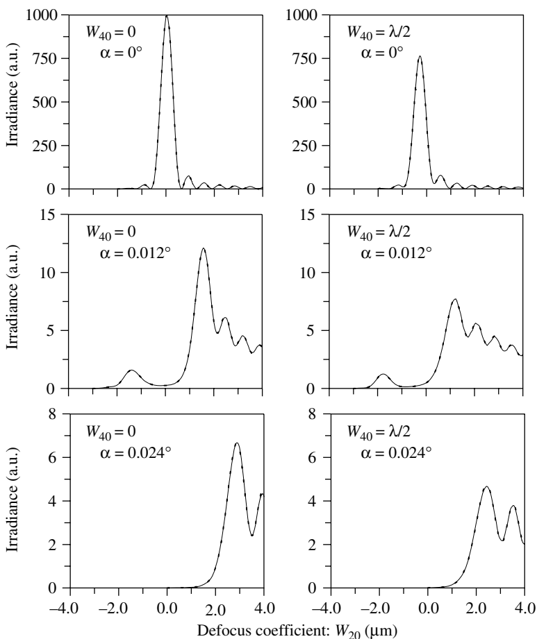
FIGURE 4.11 Irradiance values provided by system I, along different lines containing the axial point of the pupil and for two different amounts of SA. Continuous lines represent the result by the proposed RWT method while dotted lines stand for the computation by the classic method.
