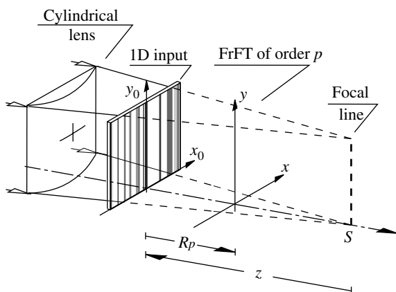
FIGURE 4.3 Implementation of the FrFT by free-space propagation.
